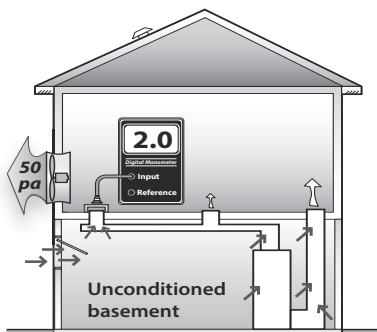
Pressure pan test: A pressure pan reading of 2 indicates moderate duct air leakage in the supply ducts.
